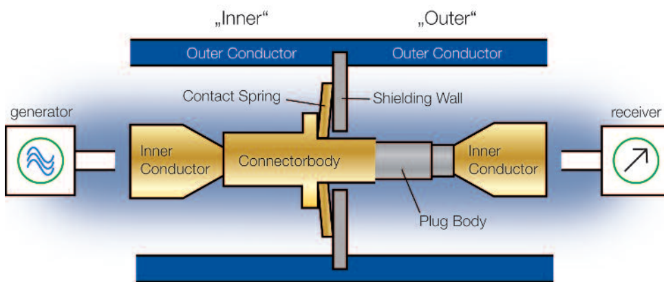
Figure 13: Measuring of EMC gaskets and feedthroughs, principle
