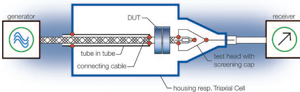
Figure 10: Triaxial Cell, principle
